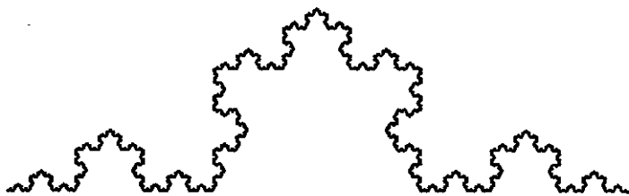
Figure 6-14 Modeling a coastline with the Koch curve.
