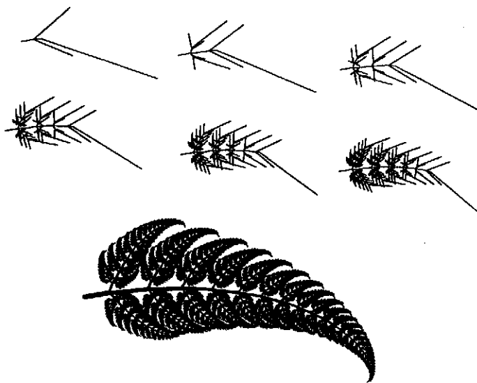
Figure 6-15 Fractal forgery of a fern; from Garcia (1991).
