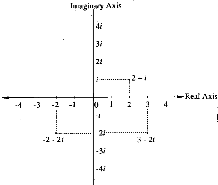
Figure 6-17 The complex plane.
