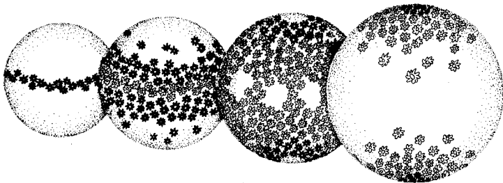
Figure 5-5 The four evolutionary phases of Daisyworld.
