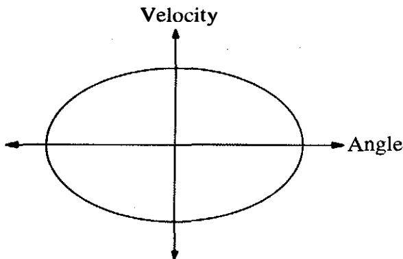
Figure 6-8 Trajectory of the pendulum in phase space.
