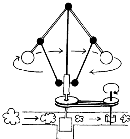
Figure 4-4 Centrifugal governor.
