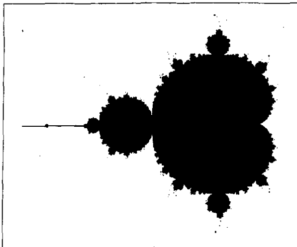
Figure 6-19 The Mandelbrot set; from Peitgen and Richter (1986).
