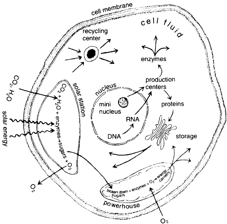
Figure 7-2 Metabolic processes in a plant cell.
