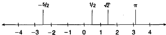
Figure 6-16 The number line.
