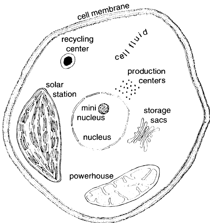
Figure 7-1 Basic components of a plant cell.
